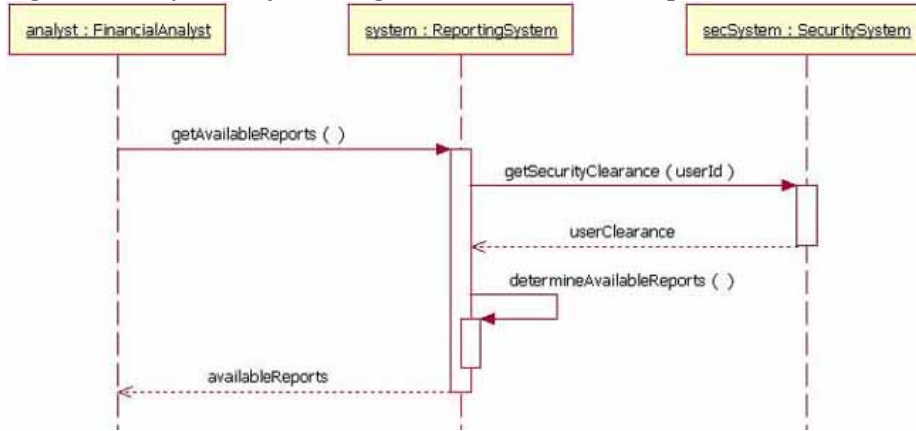
Figure 5: The system object calling its determineAvailableReports method
