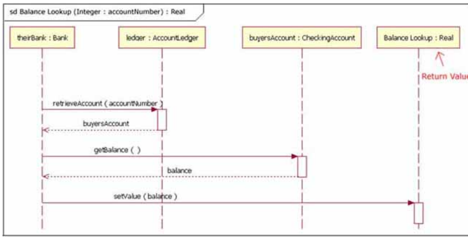
Figure 13 illustrates example 2, in which a sequence takes a parameter and returns an object. However, in Figure 13 the parameter is used in the sequence's interaction.
